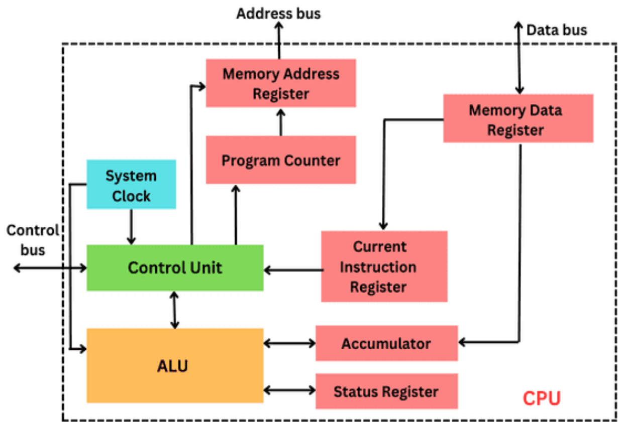
Fig: Basic components of Central Processing Unit
